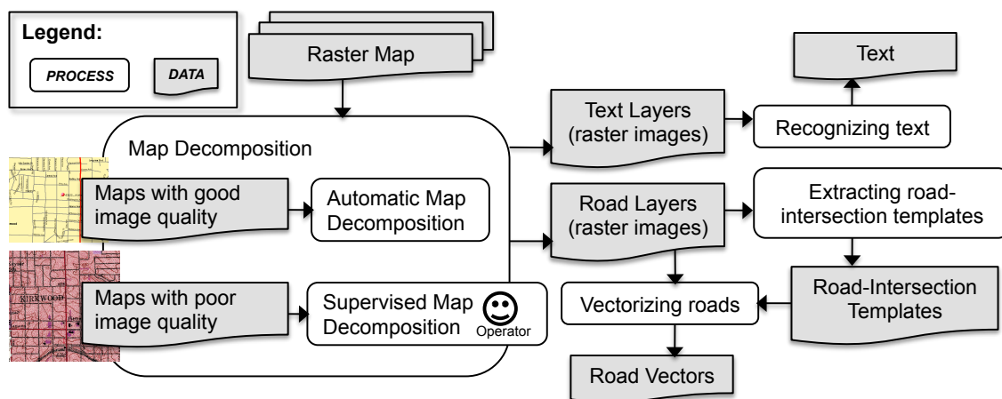
Figure 1.3: The overall approach to harvesting geographic features from heterogeneous raster maps
