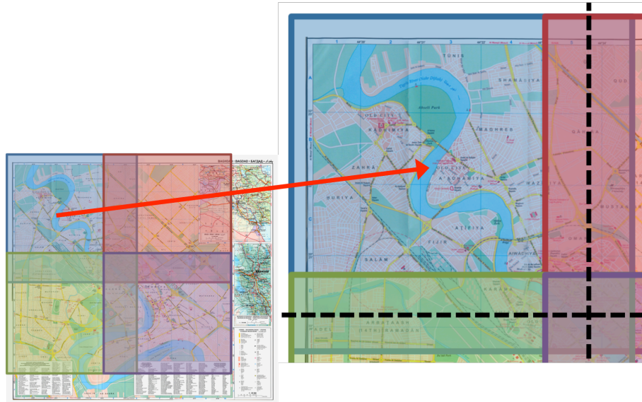
Figure 3.21: Overlapping tiles
