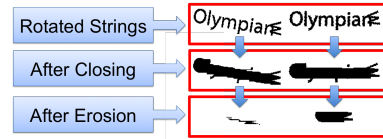
Figure 3. Detecting string orientation using morphological operators
